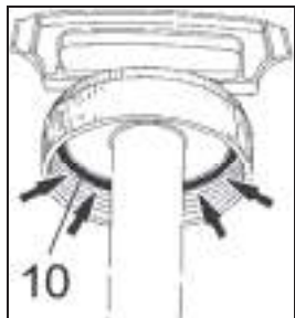
Fig. 10: For proper sealing of the spraying agent tank, the cap gasket (10) must be well greased with silicone grease.
